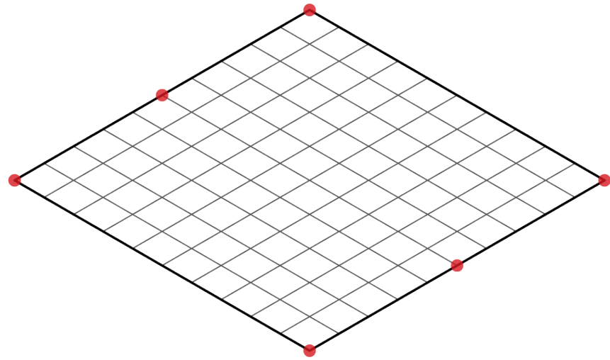
SURFACE & POINTS
