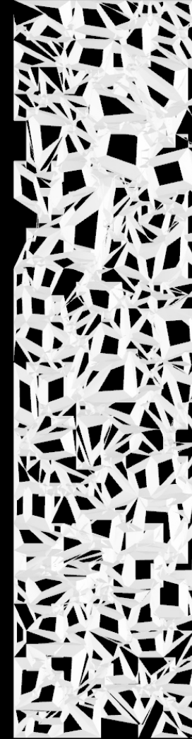
Random Attractor
