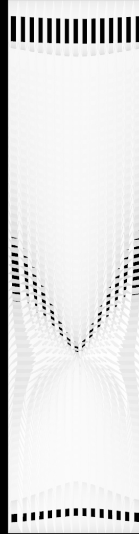
Point Attractor
