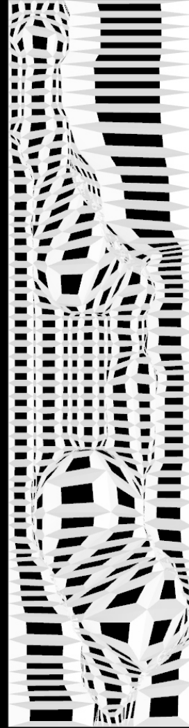
Curve Attractor
